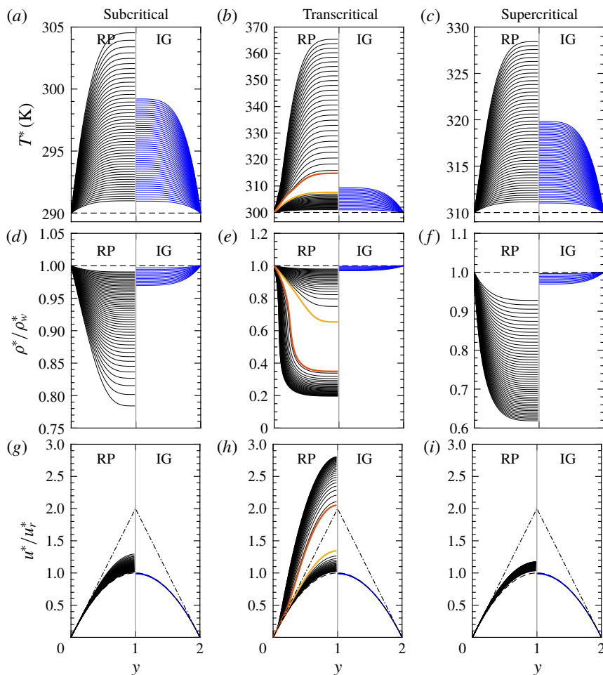
FIGURE 5. (Colour online) Temperature (a–c), density (d–f) and velocity (g–i) profiles of the base flow. The wall temperature is (a,d,g) T_w^* = 290 K, (b,e,h) T_w^* = 300 K, (c,f,i) T_w^* = 310 K respectively. PrEc increases uniformly from 0.01 to 0.1. The black and blue lines on the left and right half denote the non-ideal (RP) and ideal (IG) gases respectively. The dashed lines in each panel show the isothermal limit. The REFPROP library is used for the transport and thermodynamic properties of the non-ideal gas. The orange and red lines in panels (b,e,h) show the profiles at PrEc = 0.05115 and 0.05116 respectively. The dash-dotted lines (the triangle) in (g,h,i) show the lines of constant gradient |\partial u/\partial y| = \hat{F} .
