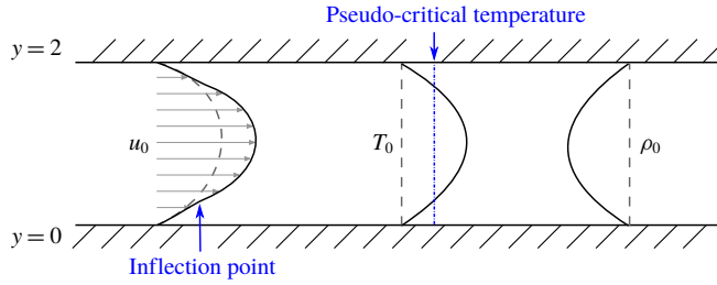
FIGURE 3. (Colour online) Sketch of the laminar base flow. Dashed lines show the isothermal limit with PrEc \rightarrow 0 , such that u_0 = y(2 - y) , T_0 = 1 , \rho_0 = 1 . Solid lines represent a transcritical case, in which T_0 crosses T_{pc} and u_0 is inflectional.
