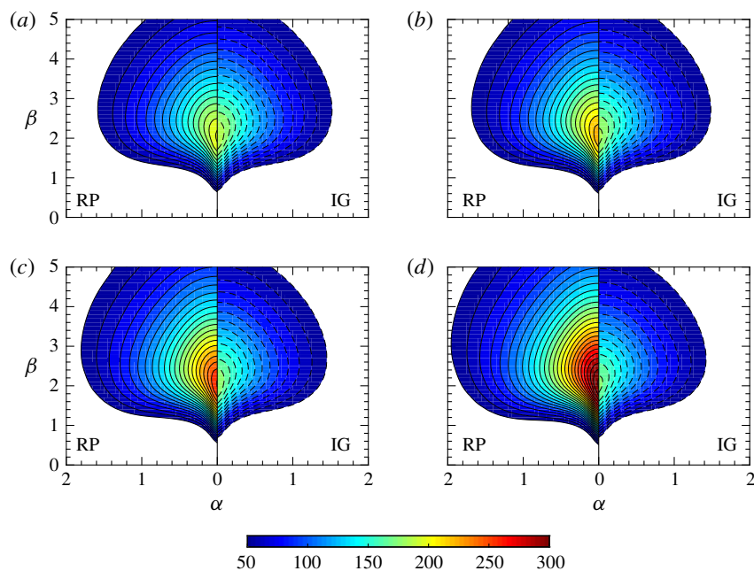
FIGURE 12. (Colour online) Contour plot of G_{max} at T_w^* = 290 K. Re = 1000 . On the left- and right-hand side of each panel, we show the results for non-ideal (RP) and ideal (IG) gases respectively. (a) PrEc = 0.01 , (b) PrEc = 0.03 , (c) PrEc = 0.05 , (d) PrEc = 0.07 .
