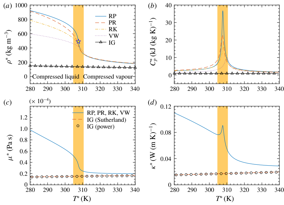
FIGURE 2. (Colour online) Thermodynamic and transport properties of CO 2 at p^* = 80 bar for the fluid models in table 1. Distribution of (a) density \rho^* , (b) heat capacity at constant pressure C_p^* , (c) viscosity \mu^* and (d) thermal conductivity \kappa^* versus temperature T^* . The pentagram shows the pseudo-critical temperature T_{pc}^* (RP model). The shaded area indicates the pseudo-critical transition.
