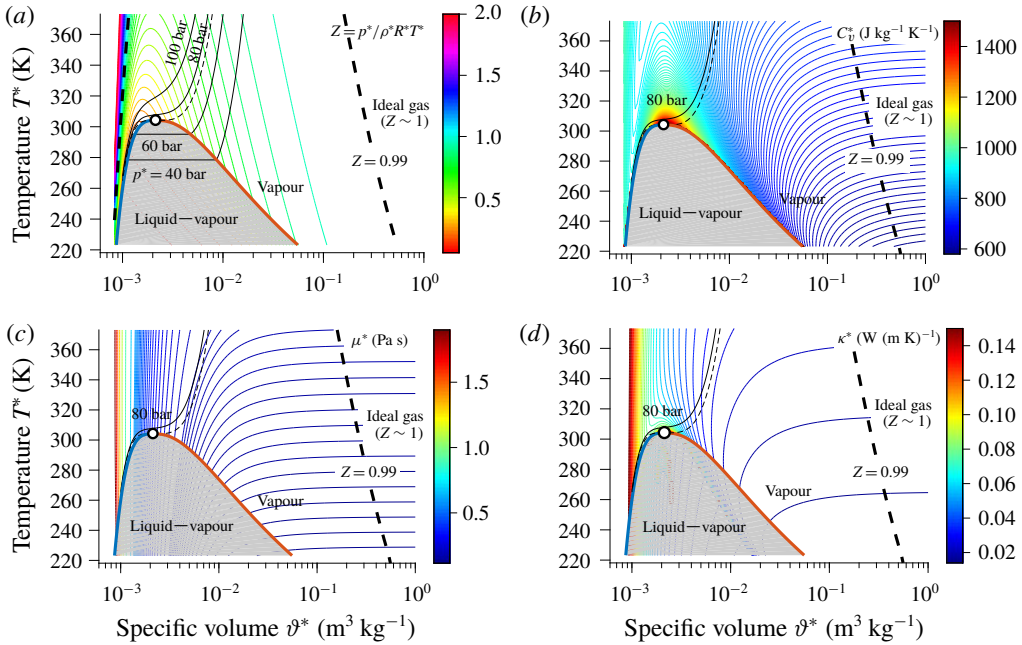
FIGURE 1. (Colour online) T – \vartheta diagram of \text{CO}_2 along with the critical point (white circle), the saturation curves (blue and red solid lines), the liquid–vapour region (grey area), the critical isobar (black thin dashed line), isobars of 40, 60, 80 and 100 bar (black thin lines), compressibility factor Z = 0.99 (black thick dashed line) as well as coloured contour lines of (a) Z = p^*/\rho^*R^*T^* , (b) the specific heat capacity at constant volume C_v^* , (c) the dynamic viscosity \mu^* , and (d) the thermal conductivity \kappa^* .
