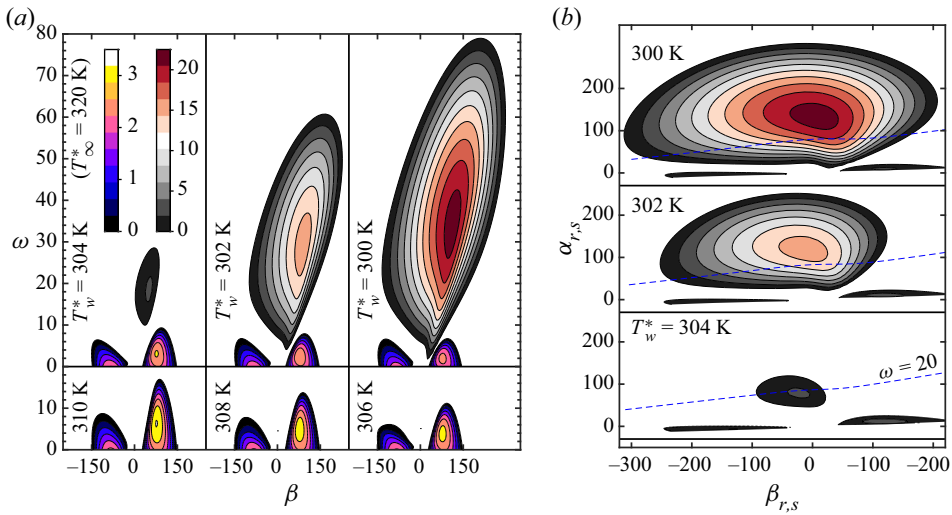
Figure 14. Stability diagram of the transcritical regimes at x = 1 . (a) Cases with T_w^* = 310, 308, 306, \dots, 300 K; (b) cases with T_w^* = 304, 302 and 300 K (shown in the \alpha_{r,s} - \beta_{r,s} coordinate). The blue dashed line gives the constant frequency \omega = 20 .
