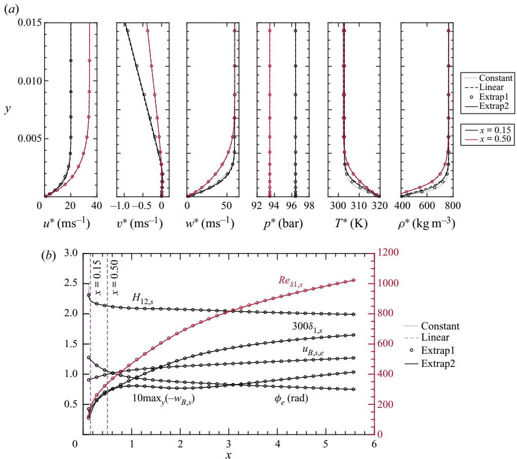
Figure 21. The PNS results obtained with different initial conditions. (a) Profiles at x = 0.15 and 0.50 ; (b) baseflow parameters as functions of x .
