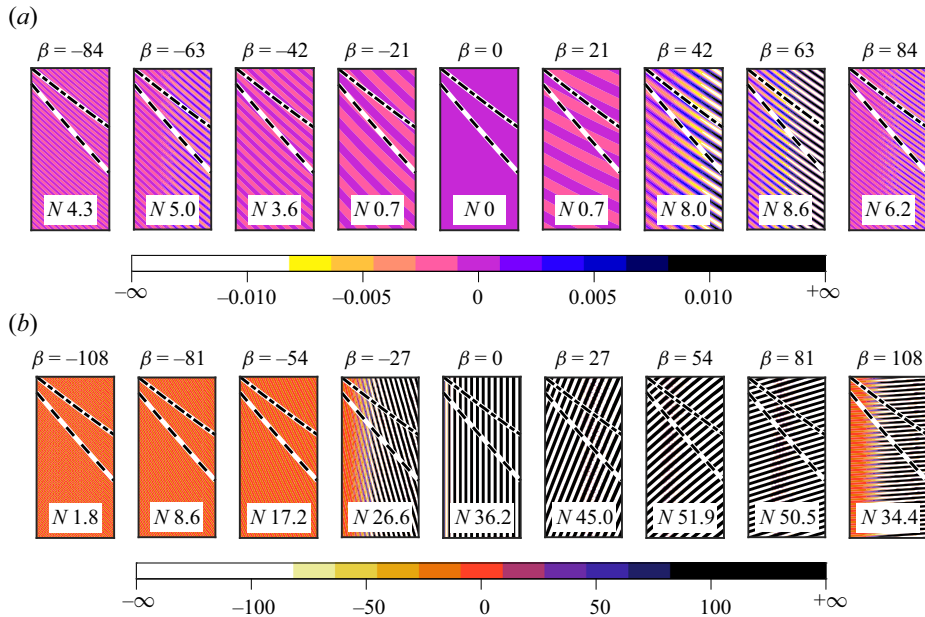
Figure 19. Display of physical perturbations \partial u'/\partial y|_{y=0}(x, z, t) for chosen spanwise wavenumber \beta . The maximum N factors at x = 5 are written at the bottom of each subpanel. (a) Wall heating and \omega = 3 , x \in [2, 3] , z \in [0, 2.08] ; (b) wall cooling and \omega = 20 , x \in [2, 3] , z \in [0, 2.08] . Movies showing the temporal evolution are available as supplemental materials.
