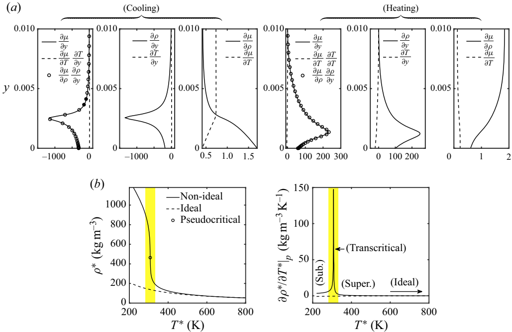
Figure 16. (a) The y-gradient of viscosity in the transcritical regimes with wall cooling and heating; (b) density \rho^* and its gradient \partial \rho^*/\partial T^*|_p versus temperature at p^* = 80 bar. The yellow shaded area stands for strong gradients of thermodynamic properties near the Widom line (pseudocritical point).
