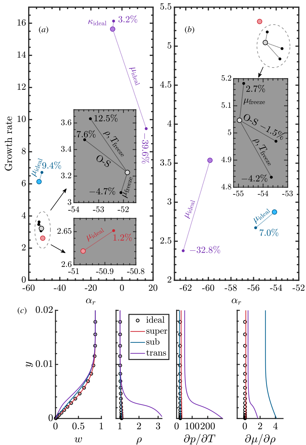
Figure 3. Discrete spectrum of the linear stability corresponding to the colored dots in Fig. 2b and c, \beta = 80 , \omega = 15 . Panel (a) is for Fig. 2b, cooling wall, and panel (b) for Fig. 2c, heating wall. We consider the influence of freezing certain inputs and O-S equations in the ideal regime. The results are denoted with small solid circles with the error of growth rate labeled. In the three non-ideal regimes (red, blue, magenta), we present the influence using ideal viscosity and thermal conductivity inputs. (c) Distribution of w , \rho , dp/dT , and d\mu/d\rho as functions of \gamma for the wall-cooling case. They belong to the velocity and density profiles and thermodynamic gradients originating from the state-variable relation and the transport properties (see Fig. 1a).
