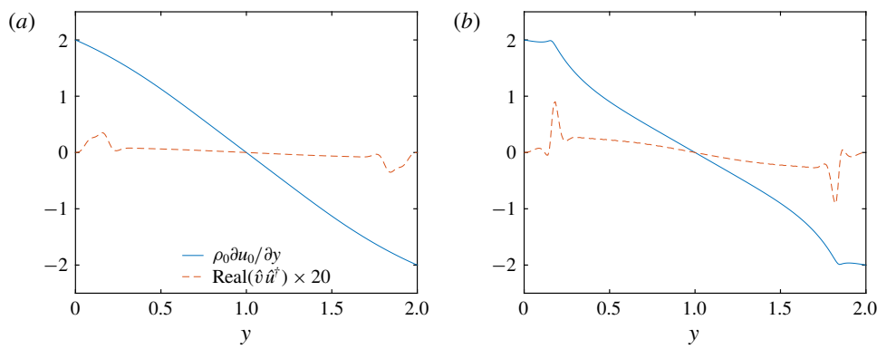
FIGURE 9. (Colour online) Production of the kinetic perturbation energy with T_w^* = 300 K, \alpha = 1 , Re = 10\,000 . (a) PrEc = 0.05 , (b) PrEc = 0.06 .
